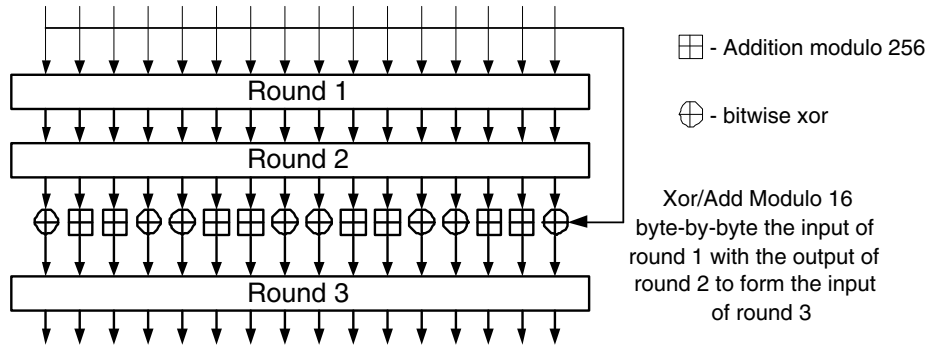
Figure 9: Combining input of round 1 with round 3 in SAFER+ modified version
